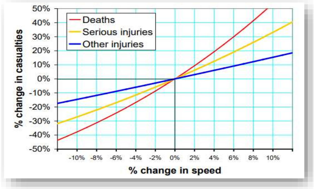
Figure 6-2: Relationship of speed changes to casualty rate changes
